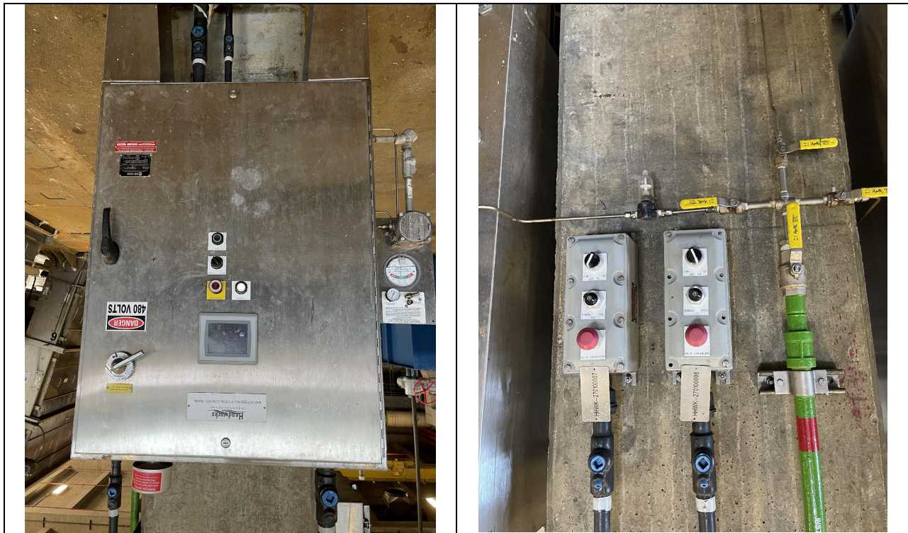
Figure 5 –Barscreen Controls
