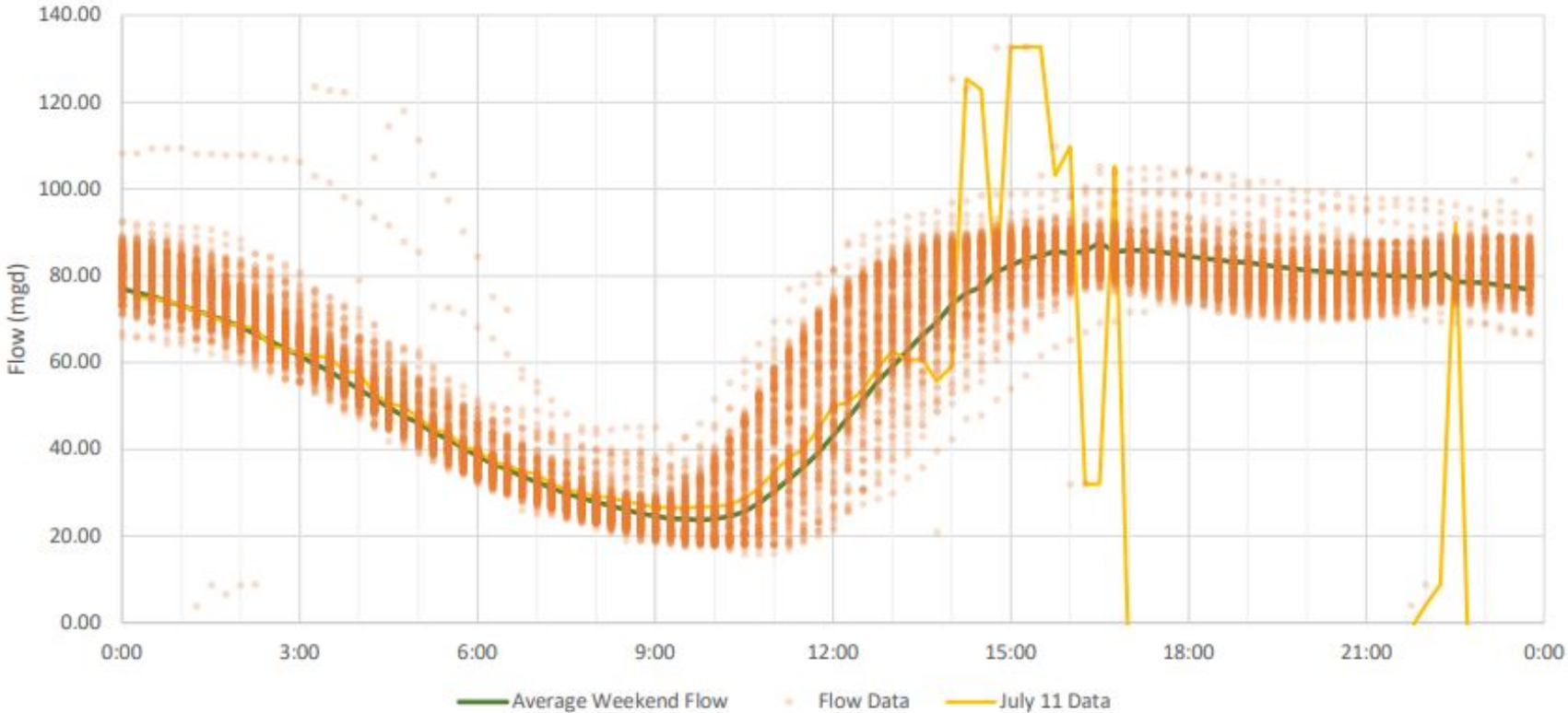
NOS - MH 56313061 Weekend Flow Pattern with July 11 Data Date Range: 01/01/2021 - 07/16/21
