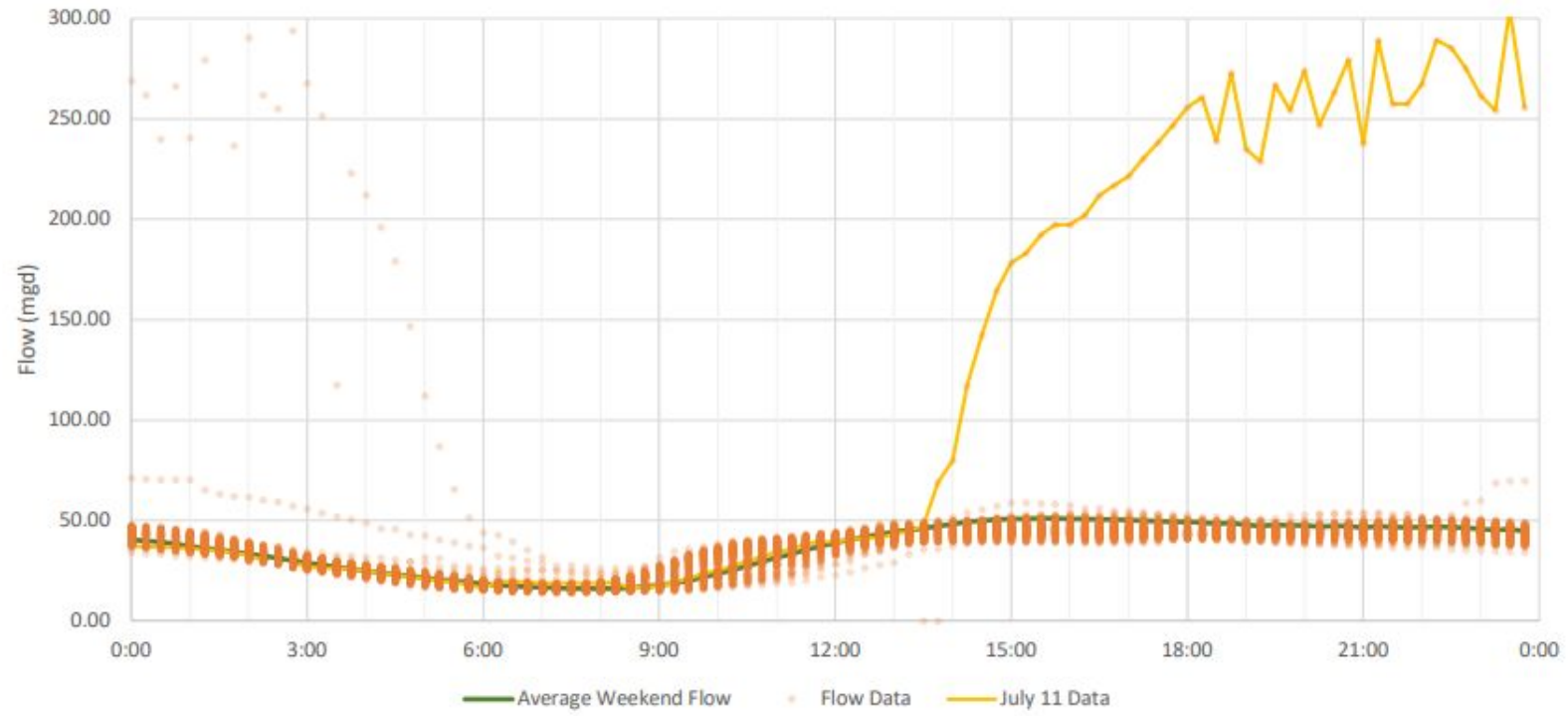
NCOS - MH 56314001 Weekend Flow Pattern with July 11 Data Data Range: 01/01/2021 - 07/16/21
