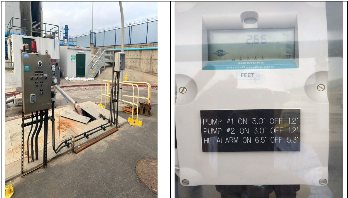
Figure 30 – CSD No. 2 (Left) and Level Sensor (Right)
