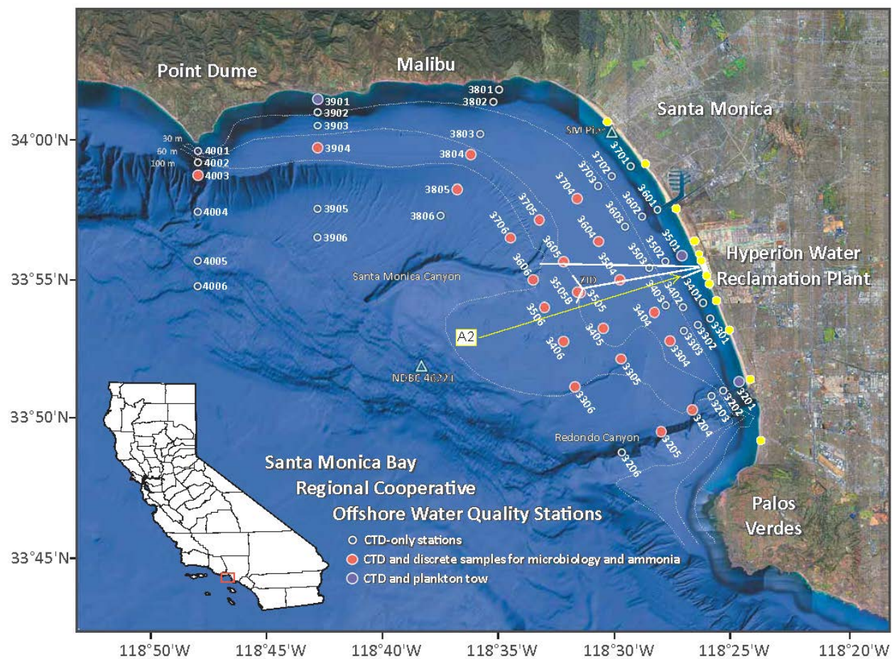
Figure 27 – Santa Monica Bay Offshore Water Quality Stations
